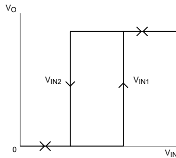
Figure 25. Non-Inverting Comparator Configuration
