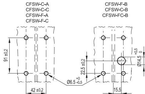
Drilling template
