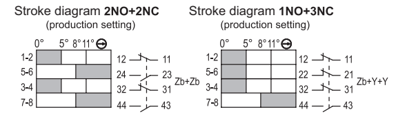
The diagrams refer to the hinge with the operating angle set in production. The operating angle can be reduced (max. adjustment: 4°).
