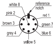
Cable/connector/extension* wiring *(see accessory on request)
