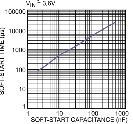
Soft-Start Time vs. Soft-Start Capacitance
