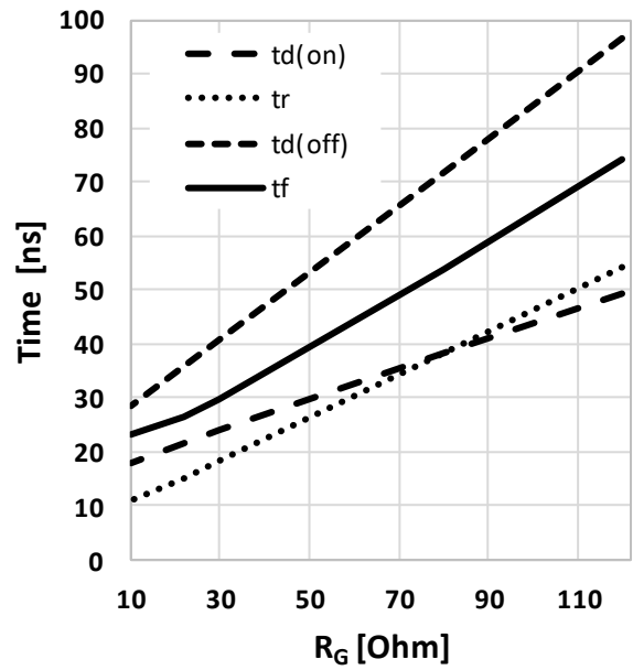
Figure 14 Typical switching times as a function of gate resistor ( t = f(R_{G,ext}), V_{DD} = 1000V, V_{GS} = 0V/12V, I_D = 2A, T_{vj} = 175^\circ C, ind. load, test circuit in Fig. E, diode: body diode at V_{GS} = 0V )
