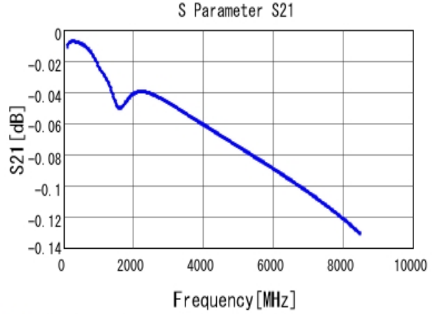
■ GRM0335C1E471GA01 S21 DCOV, 25degC
