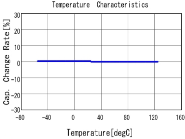
■ GRM0335C1E471GA01 C-Temp. capchange, DCOV, AC1Vrms
