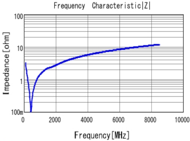
■ GRM0335C1E471GA01 |Z| DCOV, 25degC
