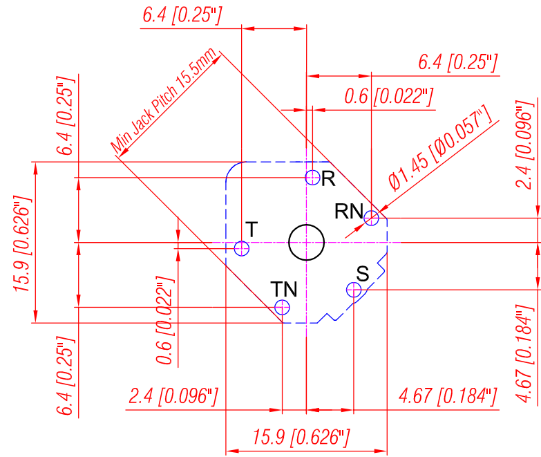
PCB LAYOUT (COMPONENT SIDE)
