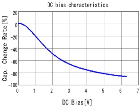
■ GRM033R60J225ME15 C-DC bias capchange, 25.0degC, AC0.
