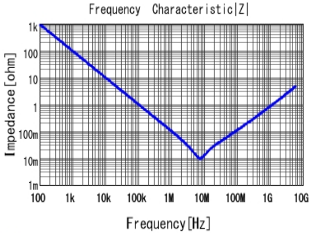
■ GRM033R60J225ME15 |Z| DCOV, 25degC
