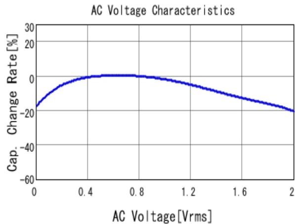
■ GRM033R60J225ME15 C-AC Voltage capchange, DCOV, 25.0d
