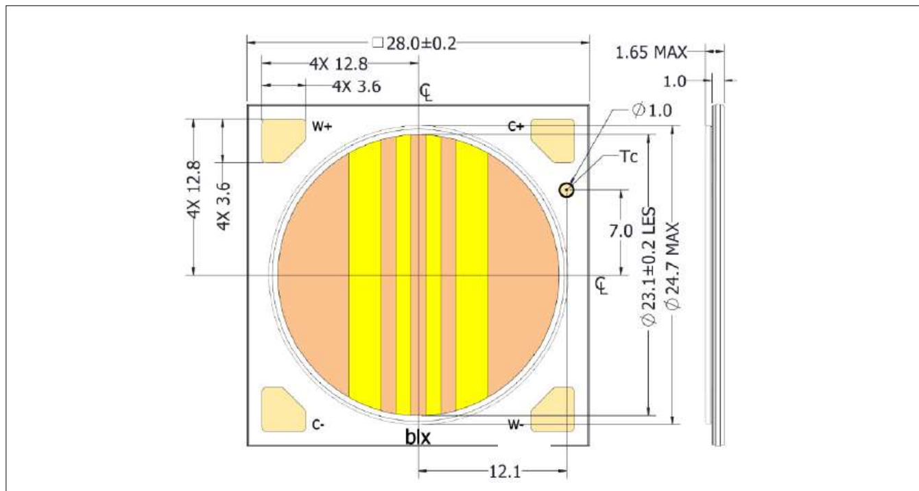
Figure 14: Drawing for Vesta Series Tunable White Gen 2 22mm Array
