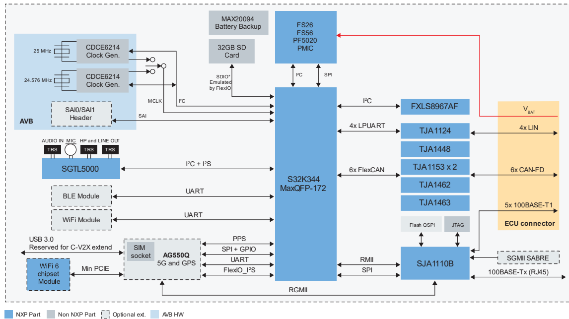
Figure 1. the Block Diagram of S32K3-T-BOX
