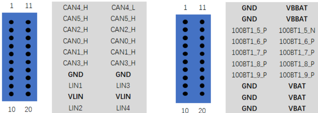
J33 ECU Connector2
