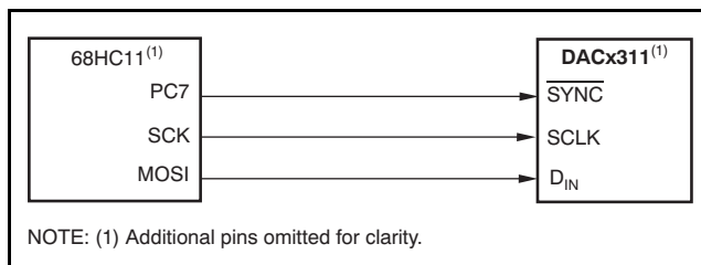
Figure 85. DACx311 to 68HC11 Interface
