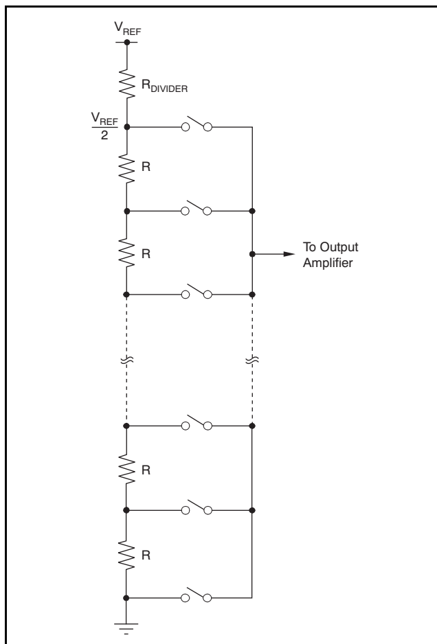
Figure 78. Resistor String
