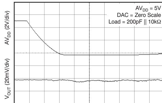
Time (10ms/div)
