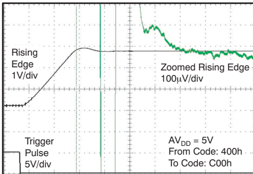
Time (2µs/div)
