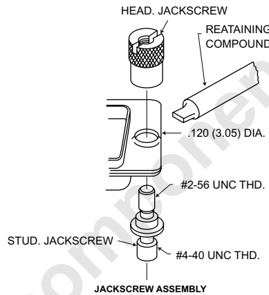
JACKSCREW ASSEMBLY
