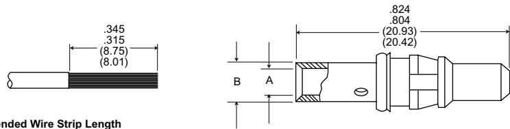
Recommended Wire Strip Length
