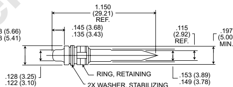
PCB Guide Pin P/N DM53745-82
