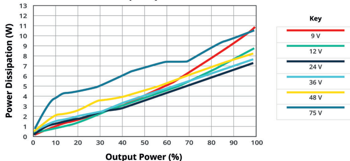
POWER DISSIPATION VS OUTPUT POWER PRQE75W-E12-S24-D (25°C)
