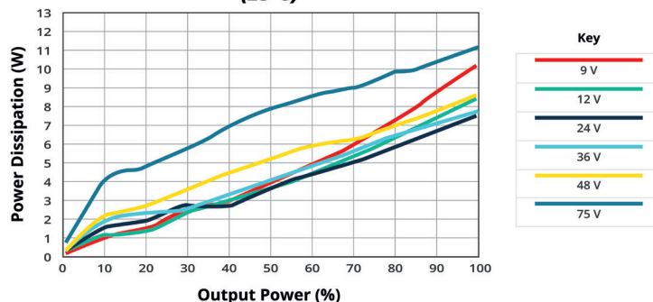
POWER DISSIPATION VS OUTPUT POWER PRQE75W-E12-S48-D (25°C)
