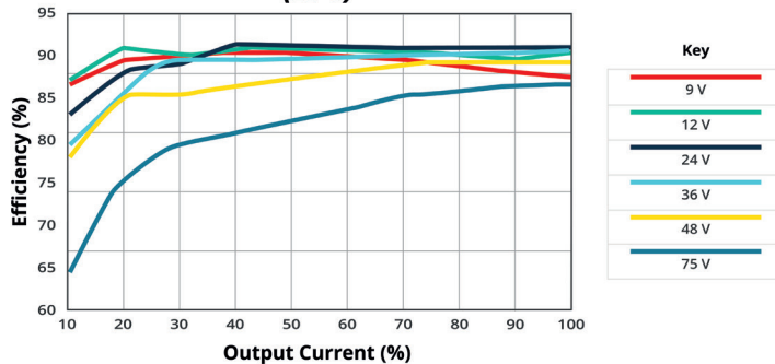
EFFICIENCY VS OUTPUT LOAD PRQE75W-E12-S28-D (25°C)
