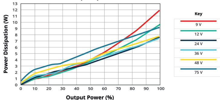
POWER DISSIPATION VS OUTPUT POWER PRQE75W-E12-S12-D (25°C)
