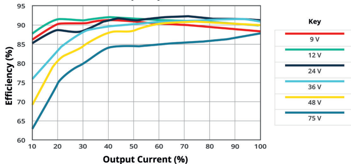
EFFICIENCY VS OUTPUT LOAD PRQE75W-E12-S48-D (25°C)
