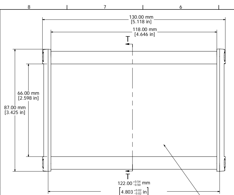
Inside Face to Face Dimension ASSEMBLY - VIEW FROM TOP
