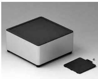
ES146059 SYNERGY S140 Aluminium AlMgSi 0,5 matt eloxiert 140x140x70mm IP 40
