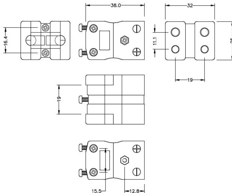
Standard Duplex in-line Socket (dimensions in mm)
