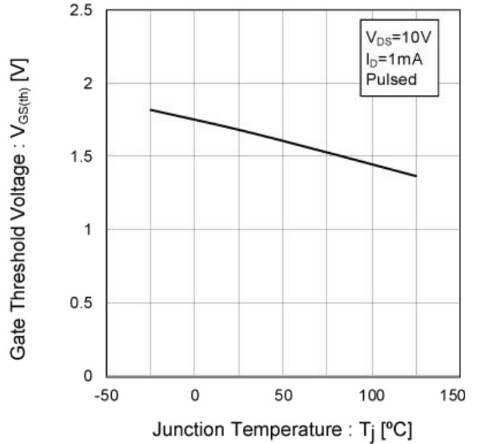
Fig.9 Gate Threshold Voltage vs. Junction Temperature
