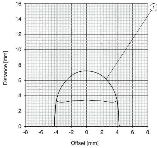
Reading range in steel IQC21-8
