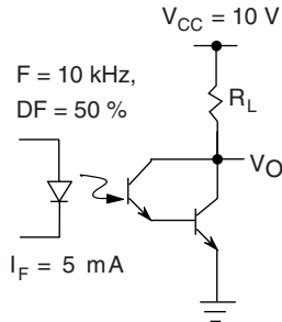
Fig. 8 - Switching Schematic
