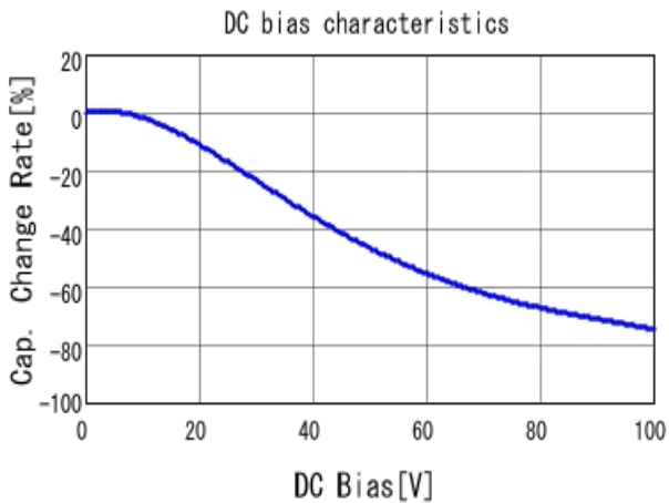
■ KRM55WR72A156MH01 C-DC bias capchange, 25.0degC, AC0.
