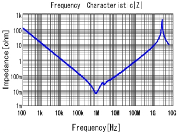
■ KRM55WR72A156MH01 |Z| DCOV, 25degC
