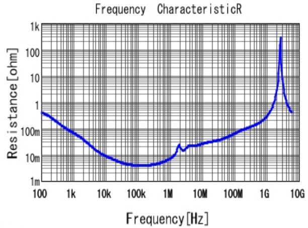
■ KRM55WR72A156MH01 R DCOV, 25degC
