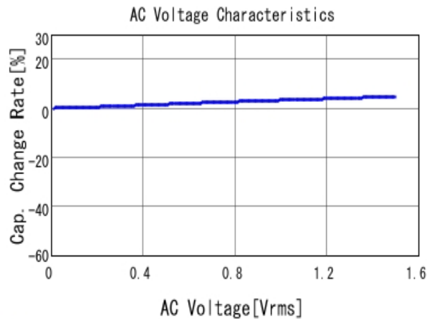
■ KRM55WR72A156MH01 C-AC Voltage capchange, DCOV, 25.0d
