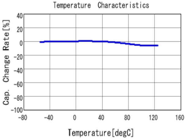
■ KRM55WR72A156MH01 C-Temp. capchange, DCOV, ACO, 5Vrms
