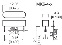
Angle of pins may deviate ± 7.5°
