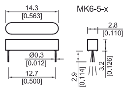
Angle of pins may deviate ± 7.5°
