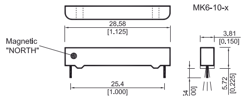
Angle of pins may deviate ± 7.5°
