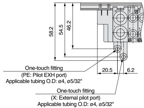
(Connector entry direction upward)
