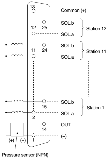
D-sub connector (25 pins)
