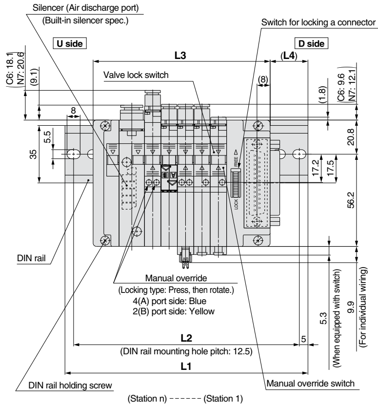
(Connector entry direction upward)
