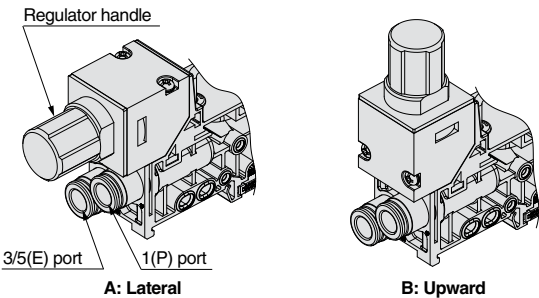
Fig.1 Handle orientation (Regulator mounting orientation)
