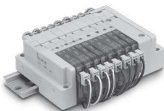
Individual wiring
