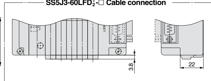
SS5J3-60FD 1/2 - Cable connection
