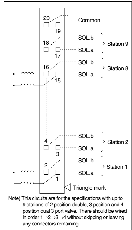
Type 60J: Flat ribbon cable (20 pins, PC wiring)
