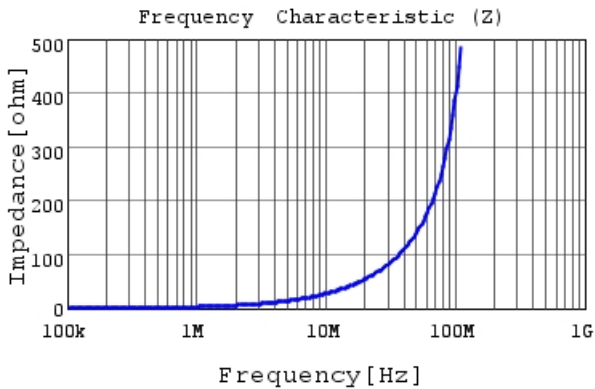
DFE18SANR47ME0 |Z|
