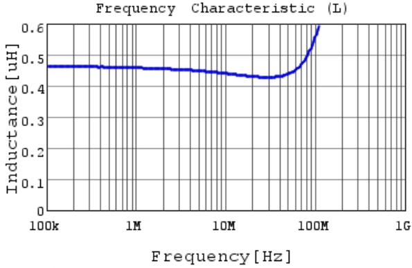
DFE18SANR47ME0 L
