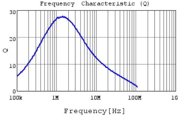
DFE18SANR47ME0 Q
