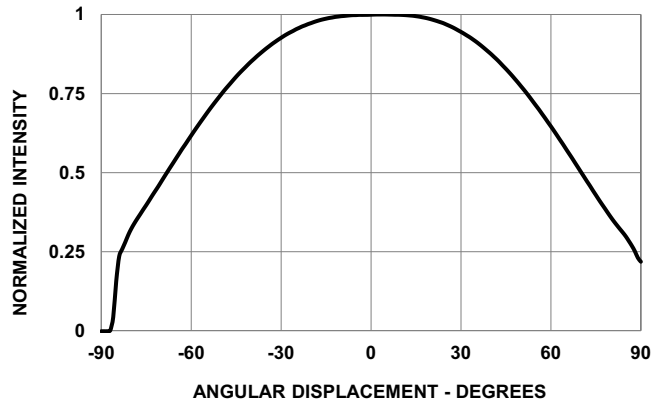
Figure 5: Radiation Pattern
