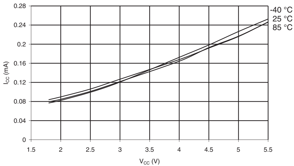
Figure 29-299. ATmega1284: Active Supply Current vs. V_{CC} (Internal RC Oscillator, 128kHz)
