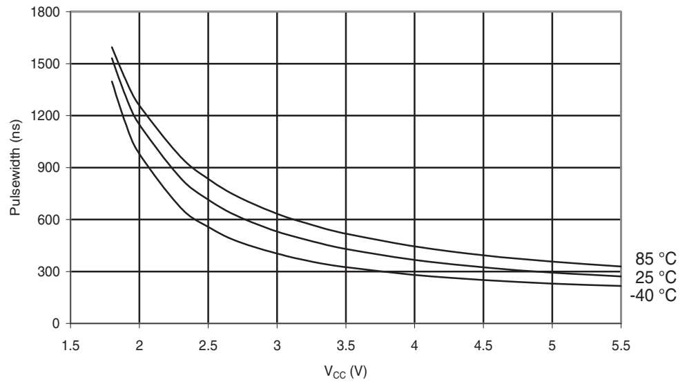
Figure 29-147. ATmega324A: Minimum Reset Pulsewidth vs. V_{CC}
