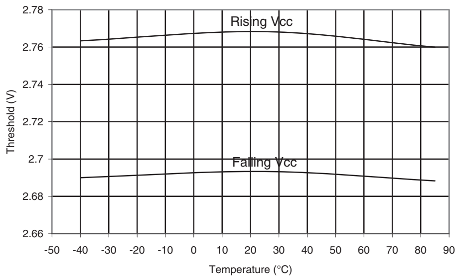
Figure 29-32. ATmega164A: BOD Threshold vs. Temperature ( V_{BOT} = 2.7V )
