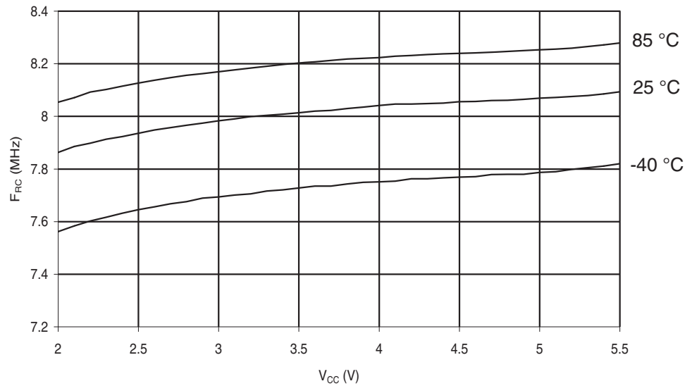
Figure 29-234. ATmega644A: Calibrated 8MHz RC Oscillator vs. V_{CC}
