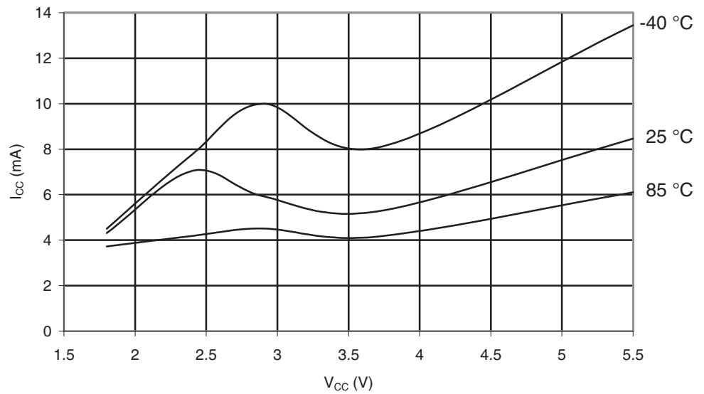
Figure 29-390. ATmega1284P: Programming Current vs. V_{CC}
