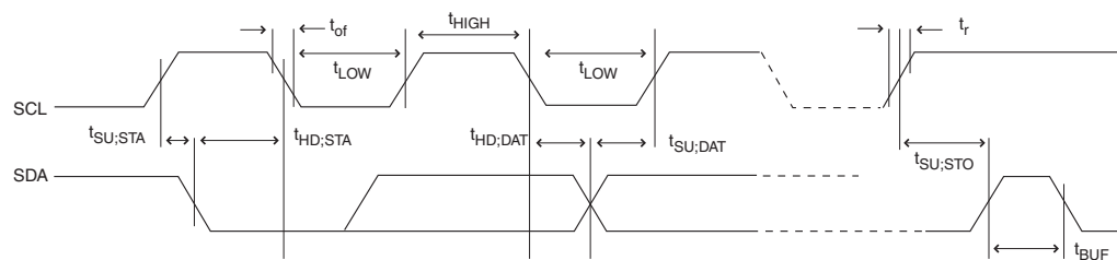
Figure 28-5. 2-wire Serial Bus Timing
