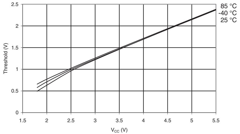
Figure 29-371. ATmega1284P: I/O Pin Input Threshold vs. V_{CC} ( V_{IL} , I/O Pin Read as '0')
