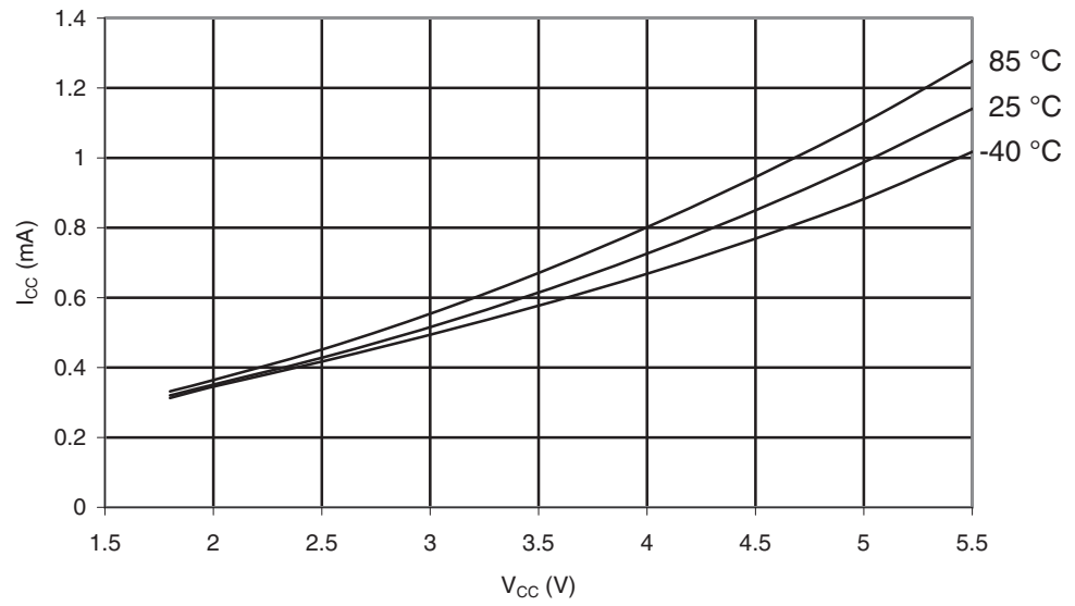
Figure 29-302. ATmega1284: Idle Supply Current vs. V_{CC} (Internal RC Oscillator, 8MHz)
