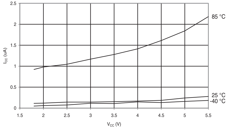
Figure 29-256. ATmega644PA: Power-down Supply Current vs. V_{CC} (Watchdog Timer Disabled).
