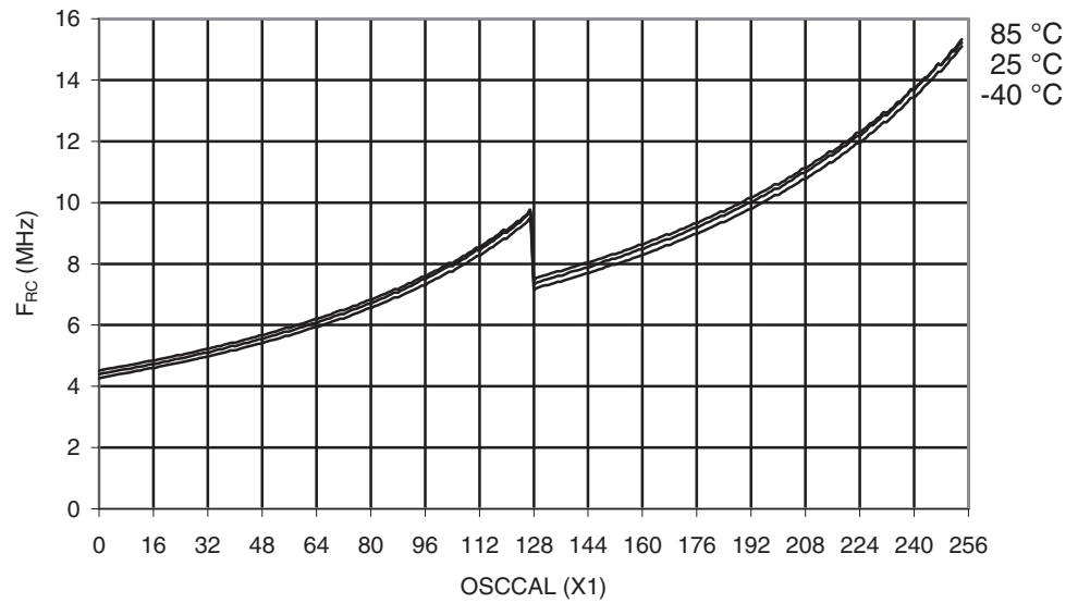
Figure 29-40. ATmega164A: Calibrated 8MHz RC Oscillator vs. OSCCAL Value
