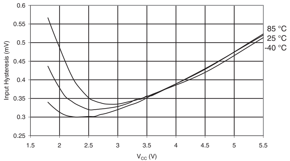
Figure 29-372. ATmega1284P: I/O Pin Input Hysteresis vs. V_{CC}
