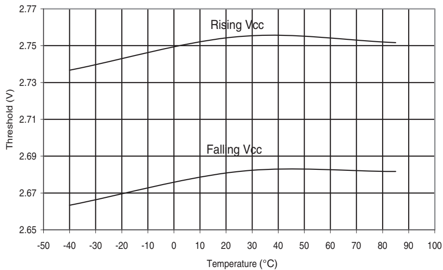
Figure 29-228. ATmega644A: BOD Threshold vs. Temperature ( V_{BOT} = 2.7V )
