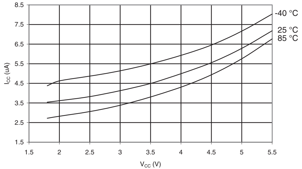
Figure 29-341. ATmega1284: Watchdog Timer Current vs. V_{CC}
