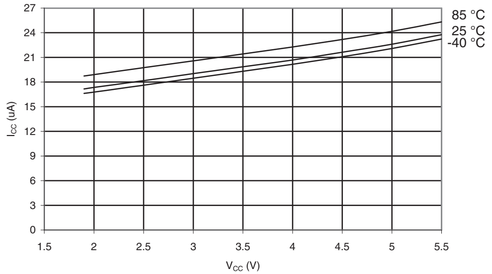
Figure 29-44. ATmega164A: Brownout Detector Current vs. V_{CC}
