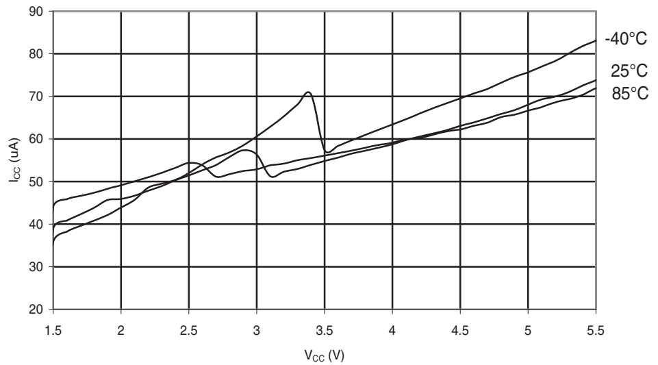
Figure 29-238. ATmega644A: Analog Comparator Current vs. V_{CC}
