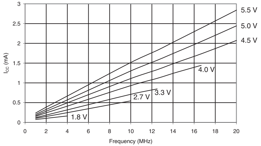
Figure 29-301. ATmega1284: Idle Supply Current vs. Frequency (1 - 20MHz)
