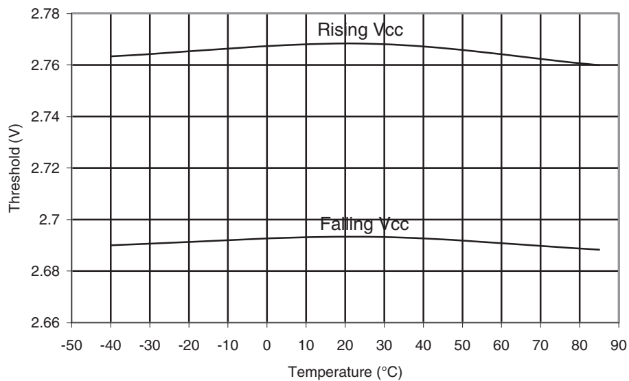
Figure 29-81. ATmega164PA: BOD Threshold vs. Temperature ( V_{BOT} = 2.7V )
