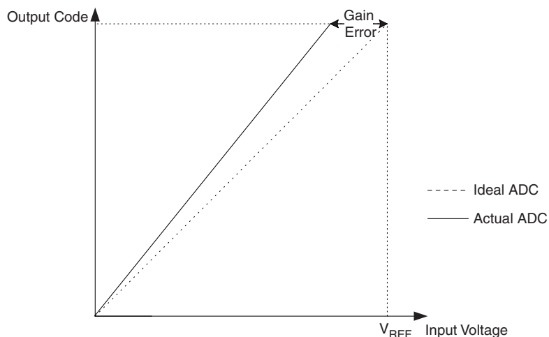
Figure 23-11. Gain Error
