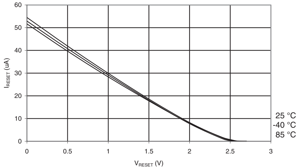
Figure 29-363. ATmega1284P: Reset Pull-up Resistor Current vs. Reset Pin Voltage ( V_{CC} = 2.7V )
