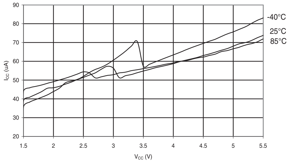
Figure 29-287. ATmega644PA: Analog Comparator Current vs. V_{CC}
