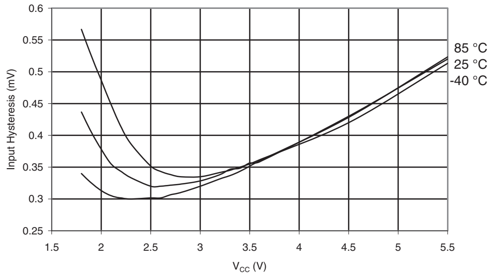
Figure 29-322. ATmega1284: I/O Pin Input Hysteresis vs. V_{CC}
