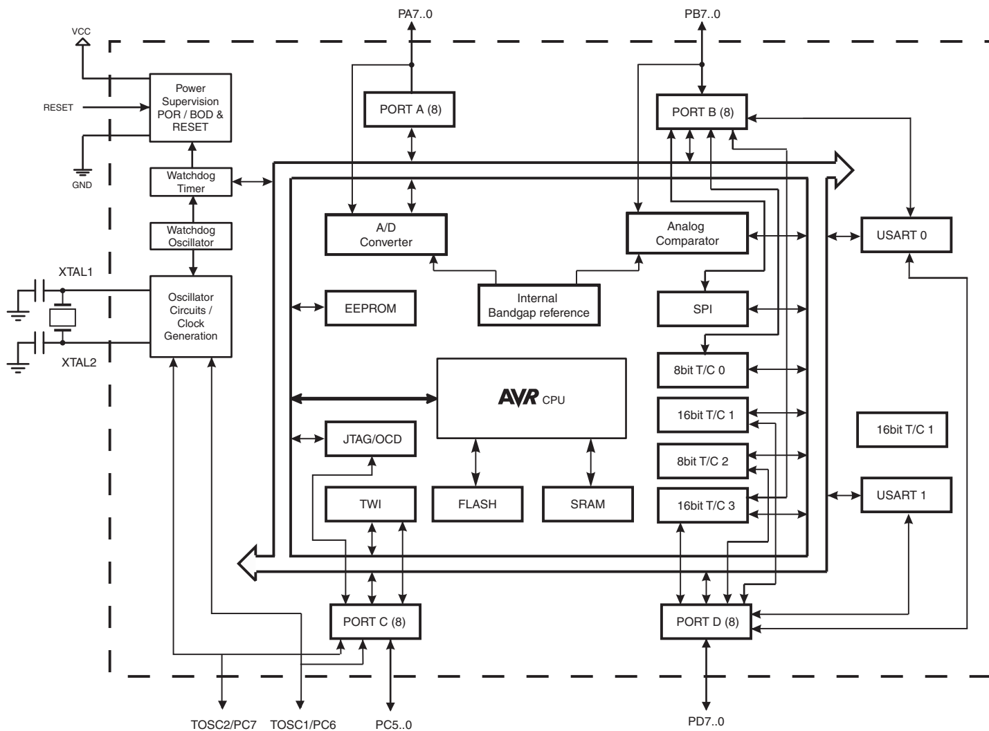
Figure 2-1. Block Diagram
