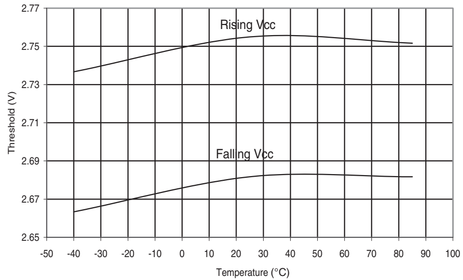
Figure 29-277. ATmega644PA: BOD Threshold vs. Temperature ( V_{BOT} = 2.7V )
