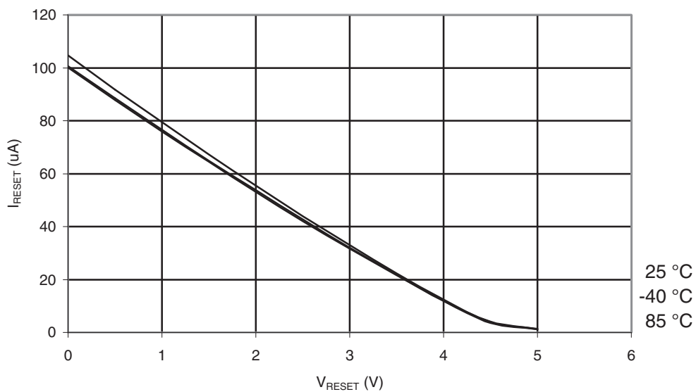
Figure 29-20. ATmega164A: Reset Pull-up Resistor Current vs. Reset Pin Voltage ( V_{CC} = 5V ).
