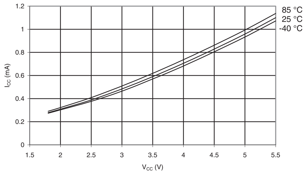
Figure 29-8. ATmega164A: Idle Supply Current vs. V_{CC} (Internal RC Oscillator, 8MHz).
