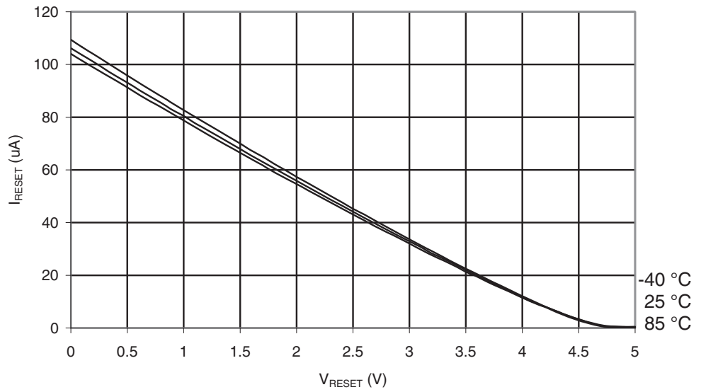
Figure 29-364. ATmega1284P: Reset Pull-up Resistor Current vs. Reset Pin Voltage ( V_{CC} = 5V )
