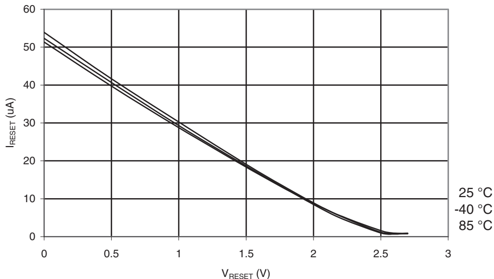
Figure 29-19. ATmega164A: Reset Pull-up Resistor Current vs. Reset Pin Voltage ( V_{CC} = 2.7V ).
