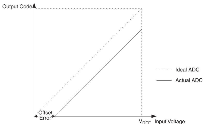
Figure 23-10. Offset Error
