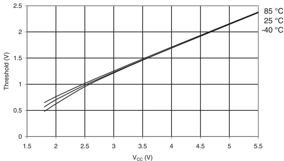
Figure 29-75. ATmega164PA: I/O Pin Input Threshold vs. V_{CC} ( V_{IL} , I/O Pin Read as '0').
