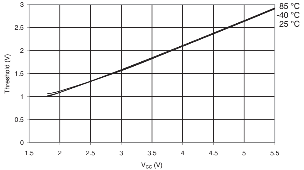
Figure 29-271. ATmega644PA: I/O Pin Input Threshold vs. V_{CC} ( V_{IL} , I/O Pin Read as '0').
