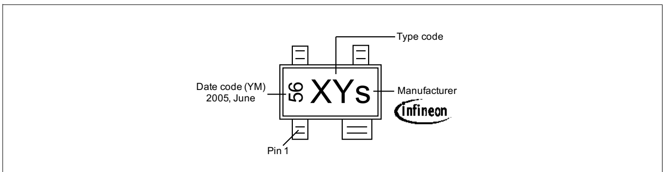
Figure 7-3 Marking Description (Marking BFP840ESD: T8s)
