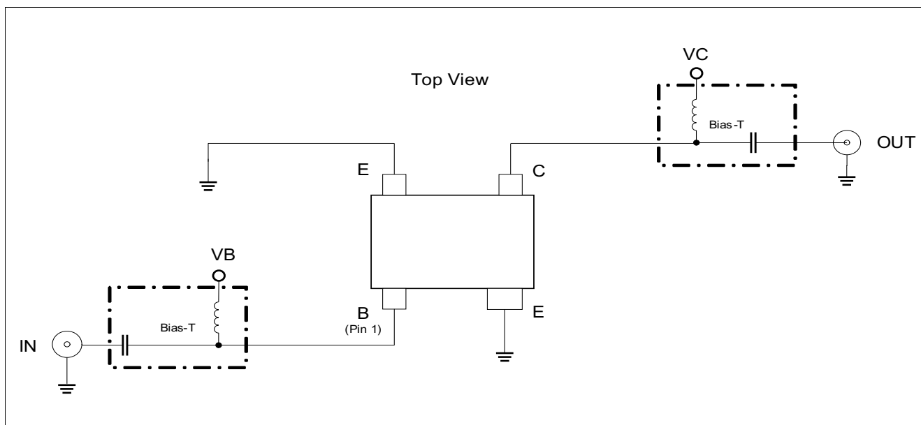
Figure 5-1 BFP840ESD Testing Circuit
