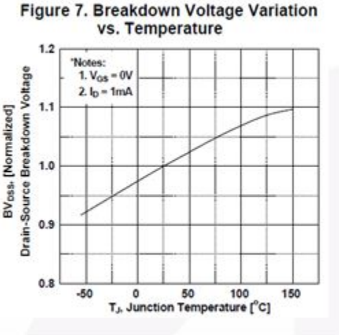
Figure 7. Breakdown Voltage Variation vs. Temperature , updated to correct for 150C temperature measurement.
