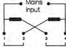
Connection Parallel 120V
