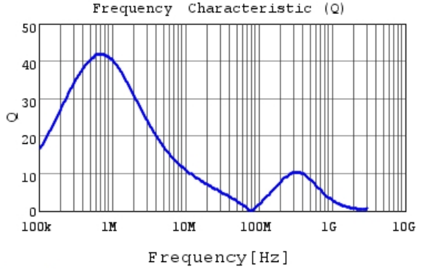
DFE2HCAH1R0MJ0 Q
