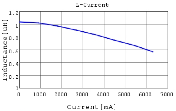
DFE2HCAH1R0MJ0 L-Current 20degC
