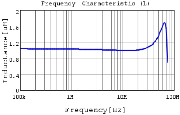
DFE2HCAH1R0MJ0 L
