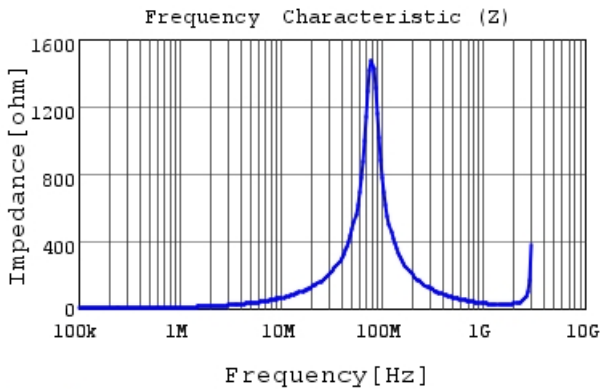
DFE2HCAH1R0MJ0 |Z|
