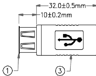
USB A Receptacle
