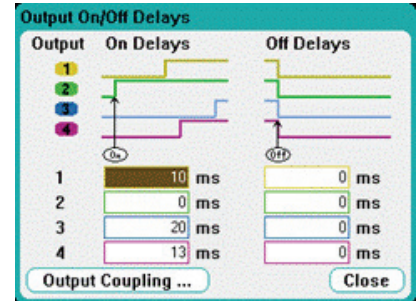
Figure 9. The Output On/Off Delays screen allows you to enter the delay times for each output. A graphical representation of the settings is shown to visually confirm your choices.
