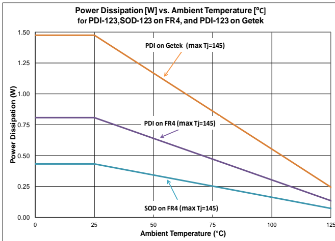
Figure 8 Power Dissipation vs. Ambient Temperature @ T_J = +145^\circ C
