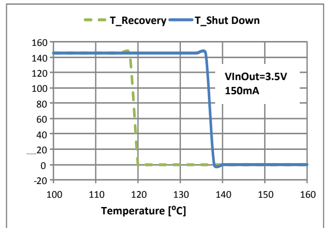
Figure 22 THSD of 150mA Current Option
