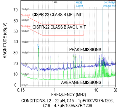
CONDUCTED EMISSIONS PLOT 5V OUTPUT, 300mA LOAD CURRENT
