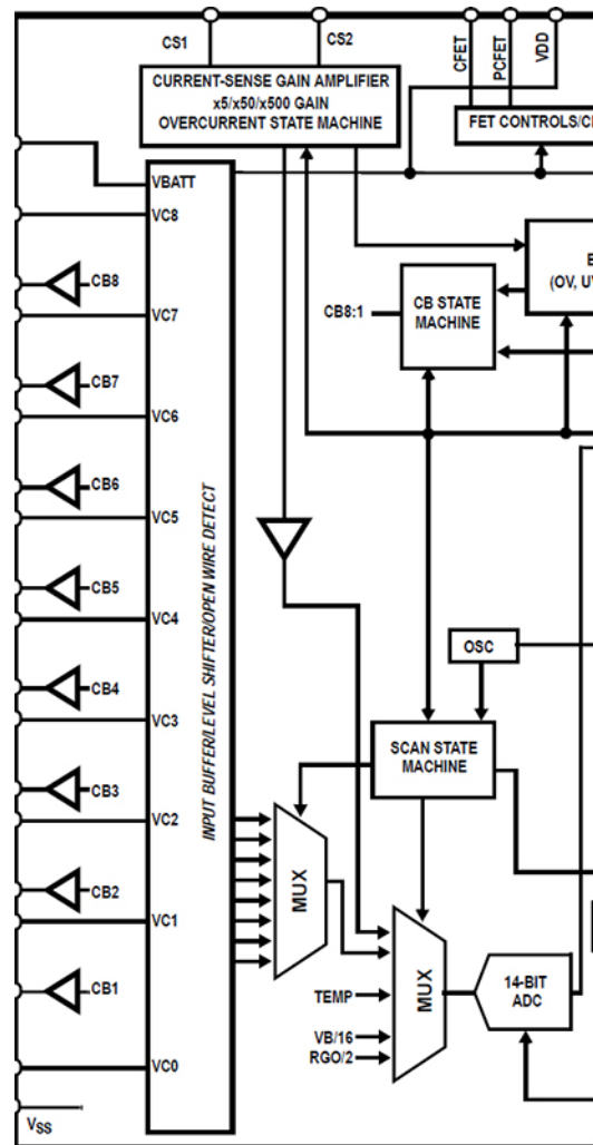
FIGURE 24. ANALOG MUX
