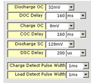
FIGURE 34. CURRENT LIMITS
