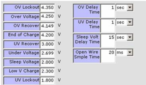
FIGURE 33. VOLTAGE THRESHOLDS AND DELAY TIMES
