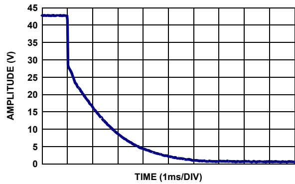
FIGURE 59. DFET FALL
