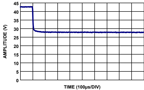
FIGURE 61. CFET FALL
