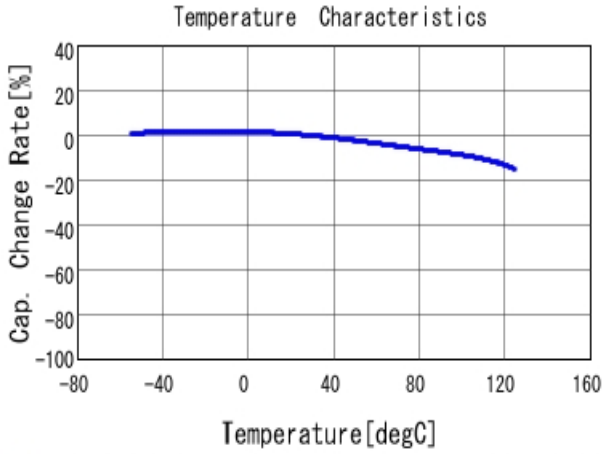
■ GCJ31CC71H475KA01 C-Temp. capchange, DC0.0V, AC1.0V r m
