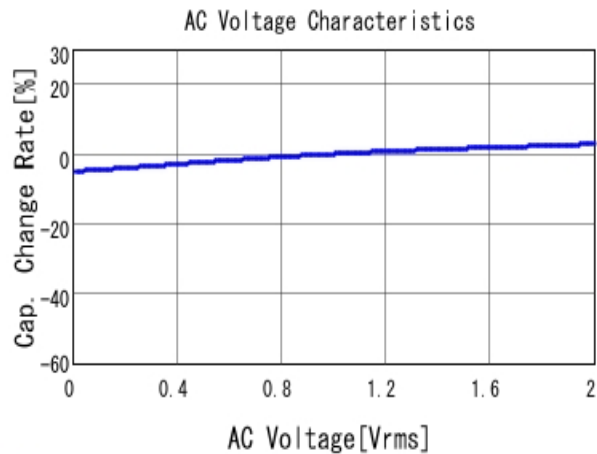
■ GCJ31CC71H475KA01 C-AC Voltage capchange, DC0V, 25.0d
