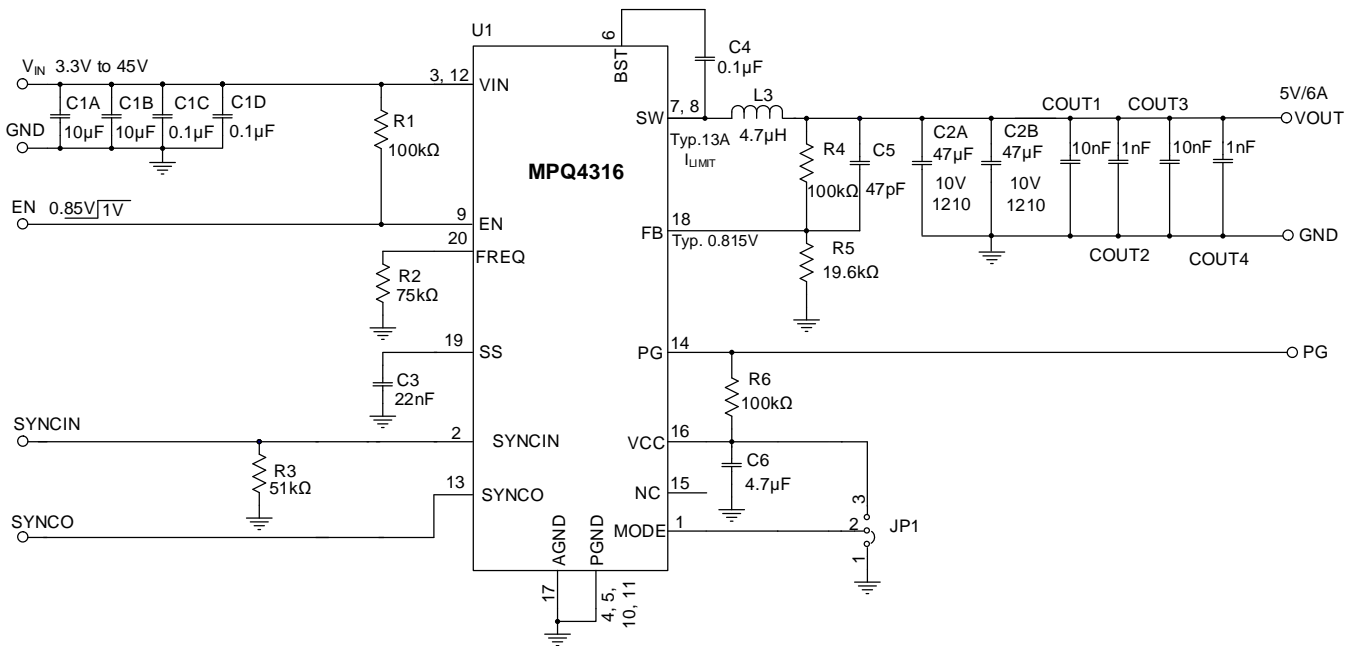
Figure 14: V OUT = 5V, f sw = 410kHz with EMI Filters
