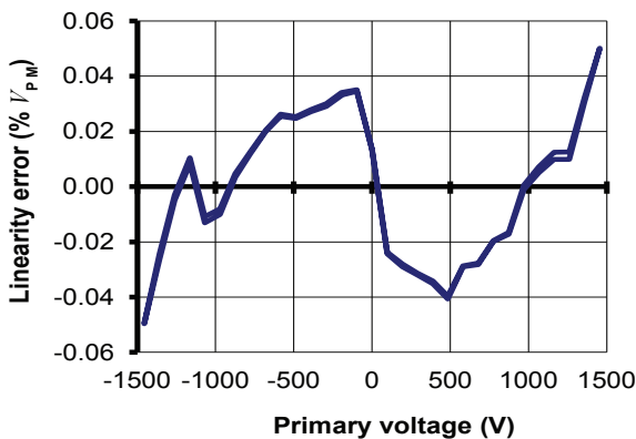
Figure 15: Typical linearity error at 25 °C
