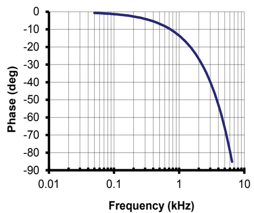
Figure 10: Typical frequency and phase response (detail)
