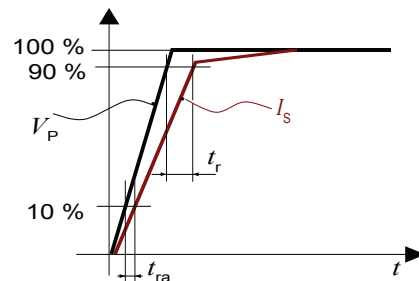
Figure 17: Response time t_r and reaction time t_{ra}
