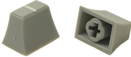
CP33041 - Slider knob CS7C Grey / White marker line Material: Polyamide
