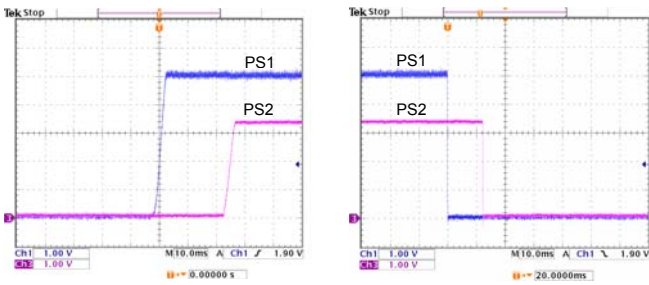
Figure 27: Sequential start-up
