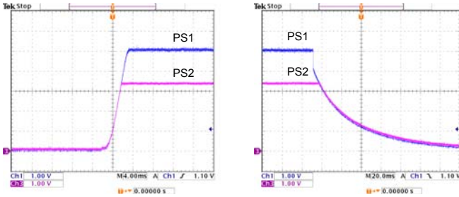
Figure 27: Sequential start-up
