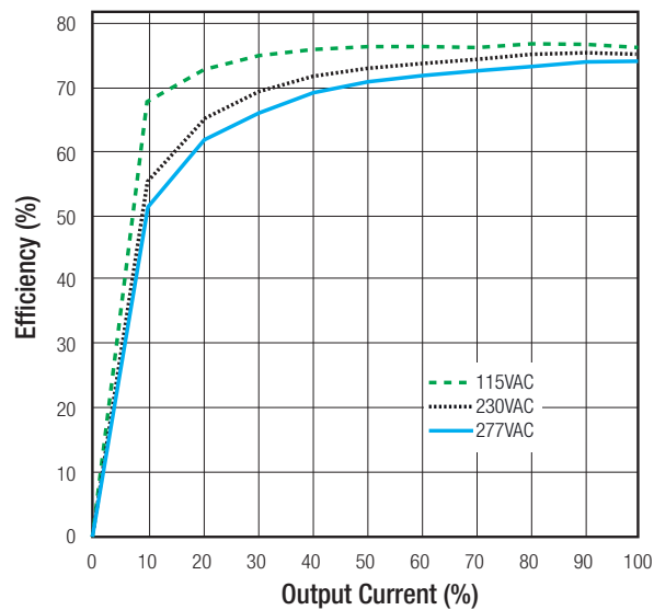
RAC04-15SC/277 (-E)
