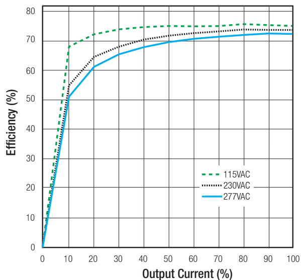
RAC04-12SC/277 (-E)
