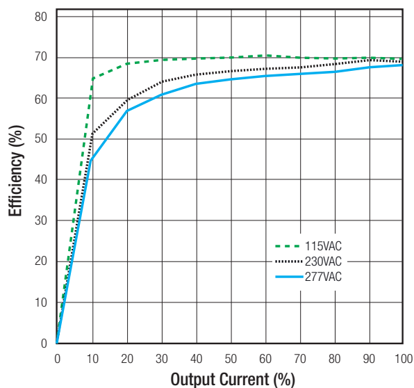
RAC04-3.3SC/277 (-E)
