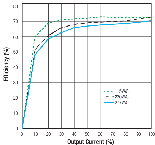
RAC04-05SC/277 (-E)
