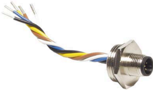
Part no.: 63000845 AC-PLM-8 Built-in plug
