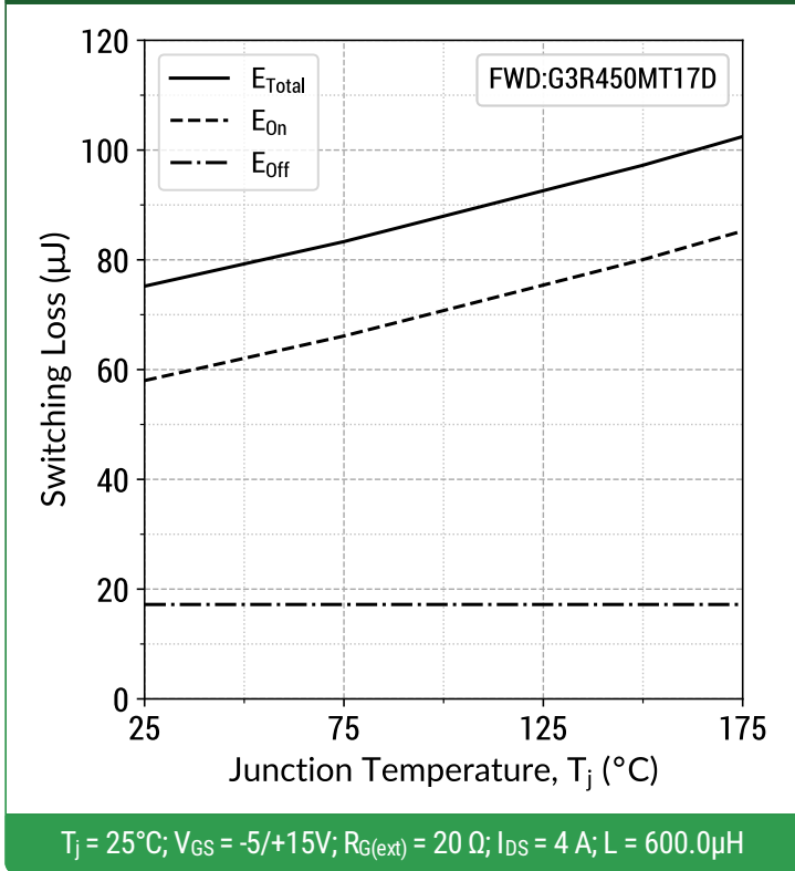
Figure 25: Inductive Switching Energy v/s Temperature ( V_{DD} = 1200V )
