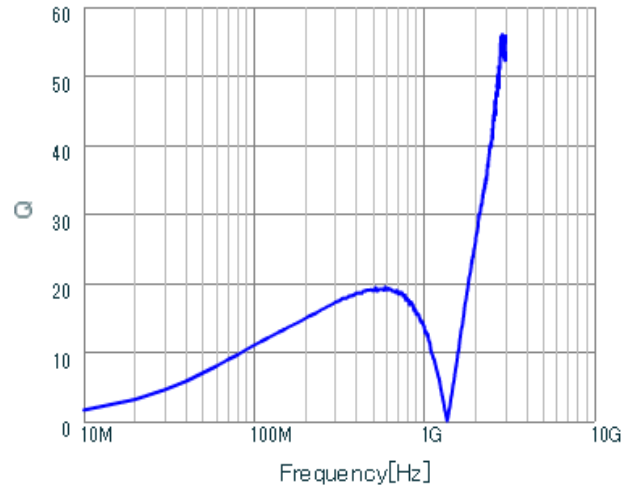
LQP03HQR12J02 Q.
