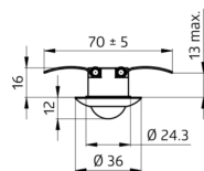
sensor head
