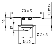
sensor head
