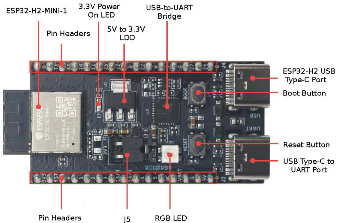
ESP32-H2-DevKitM-1 - Front
