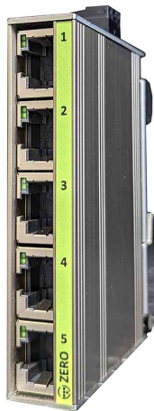
Unmanaged Industrial Ethernet Switch ZERO-RS, 5 Port
