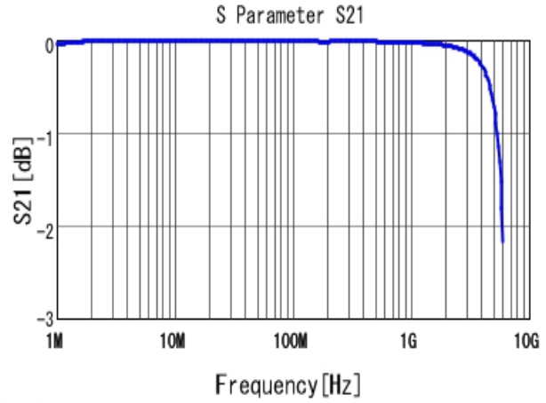
■ GRM3195C1H153JA01 S21 DCOV, 25degC
