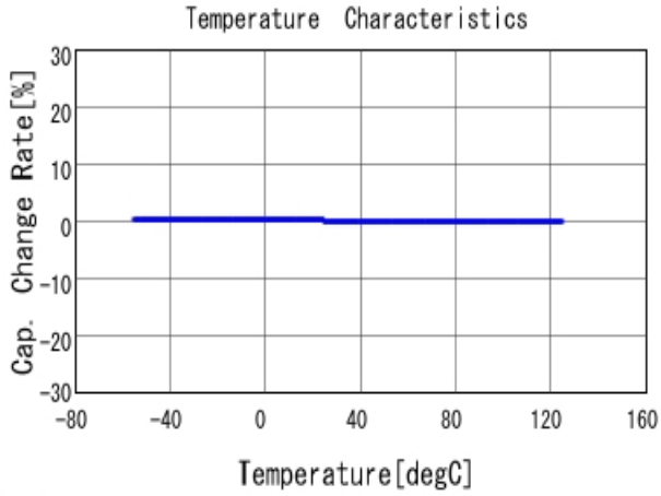
■ GRM3195C1H153JA01 C-Temp. capchange, DCOV, AC1Vrms
