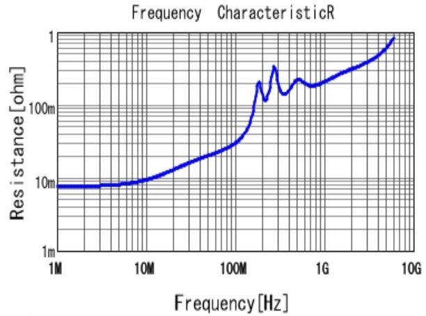
■ GRM1885C1H682JA01 R DCOV, 25degC
