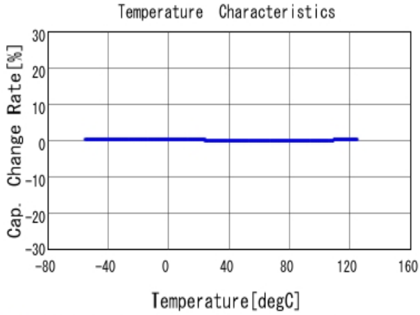
■ GRM1885C1H682JA01 C-Temp. capchange, DCOV, AC1Vrms
