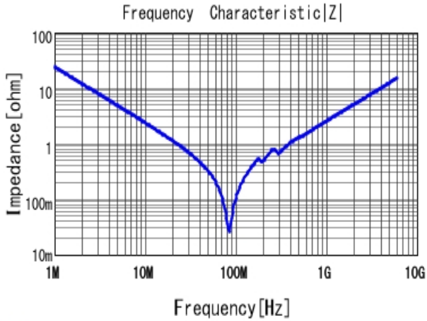
■ GRM1885C1H682JA01 |Z| DCOV, 25degC
