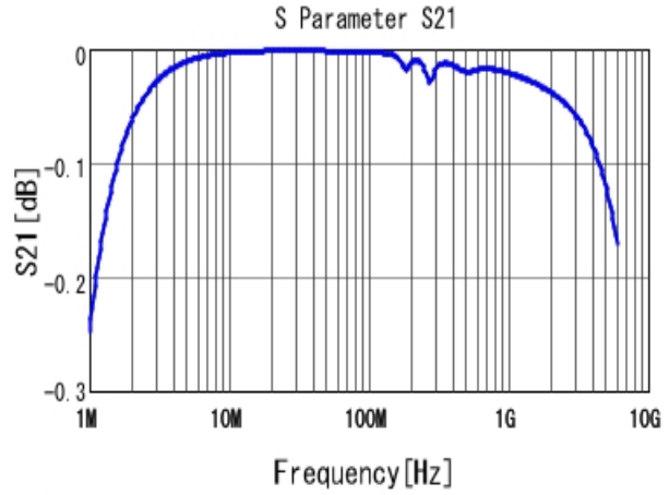
■ GRM1885C1H682JA01 S21 DCOV, 25degC
