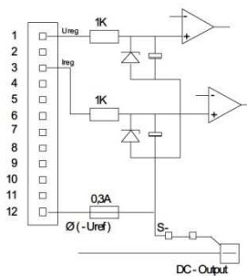
Interface Schema (Fig.3)
