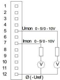
Monitor Anschlüsse (Fig.2)
