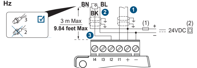
Wiring Diagram
