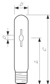
MASTER CityWhite CDO-TT Plus 50W/828 E27
